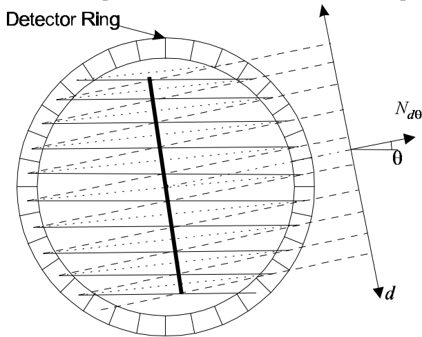
Figure 3. Sampling pattern in the transaxial plane for a PET scanner. Each segment in the detector ring represents one crystal. The solid lines show the parallel projections for the first angle, the dotted lines for the second angle, and the dashed lines for the third angle.
