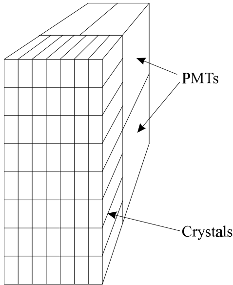
Figure 2. A block detector consisting of a 7x8 array of crystals coupled to four PMTs.
