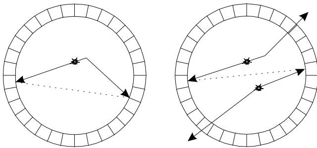
Figure 4. Diagram of a scattered event (left) and an accidental coincidence (right). Photons shown leaving the ring are scattered through an oblique angle such that their paths do not intersect a detector.
