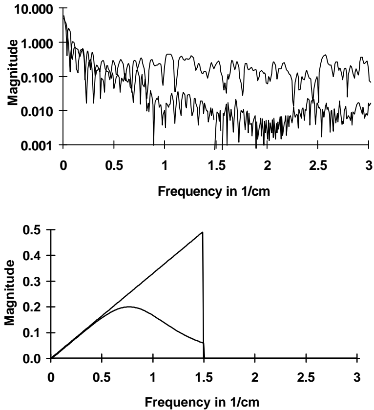
Figure 6. The magnitude spectrum of a typical projection (upper curve) and a nearly noiseless projection (bottom curve) are shown at the top. Two practical filters are shown at the bottom: a ramp filter cut off at 50% of the Nyquist rate and the same filter windowed with a Butterworth filter.
