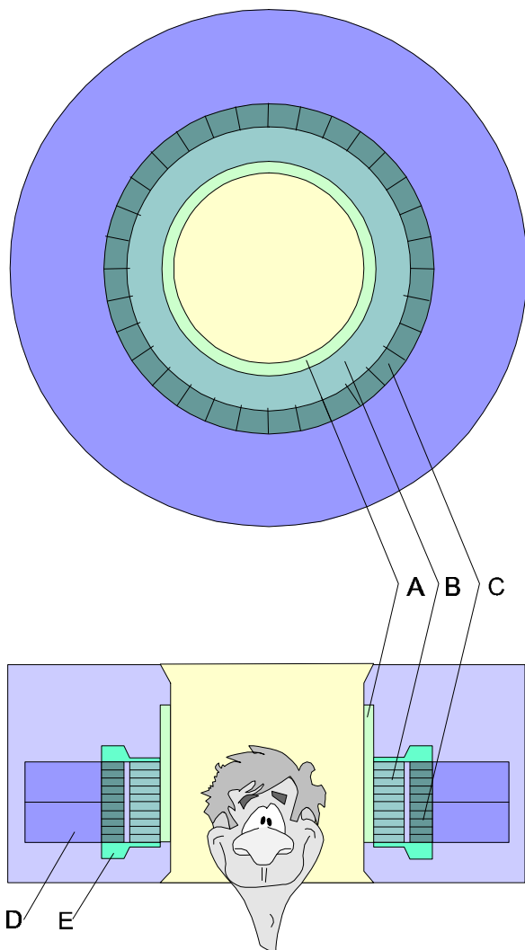
Figure 1. A transaxial view of a PET scanner (upper panel) top view (lower panel) showing the rod sources used for attenuation correction (A), the septa used for scatter reduction (B), the detector blocks consisting of crystals (C) and photomultiplier tubes (D), and the end-shields (E).
