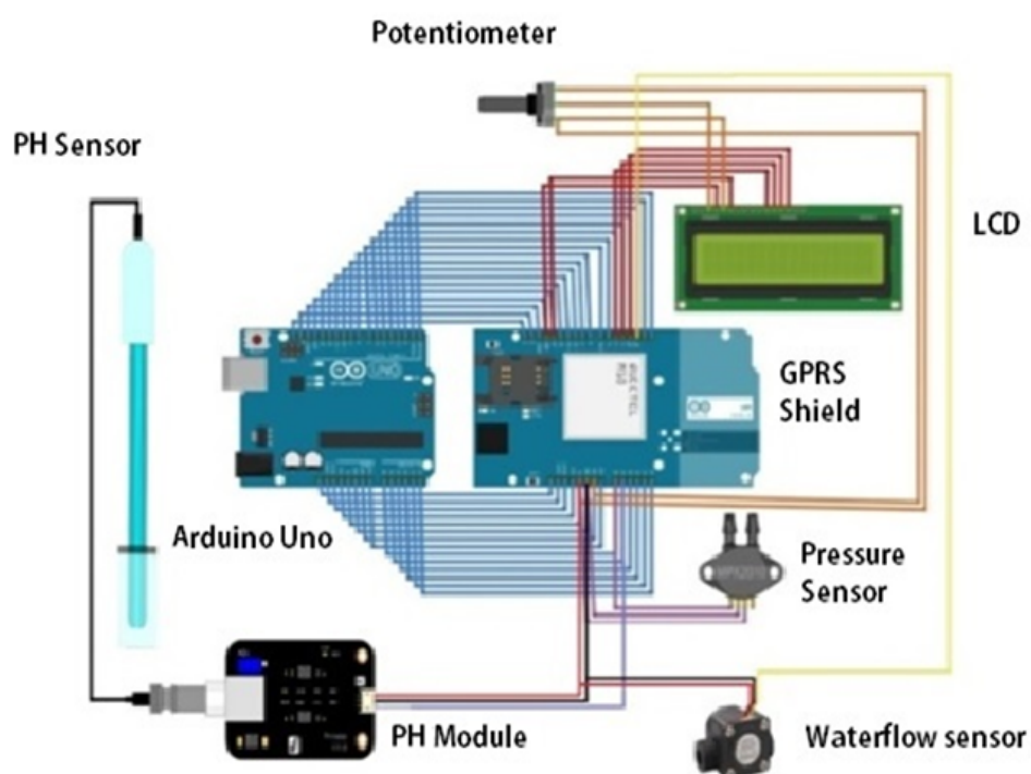
FIGURE 2. Prototype 1 design
