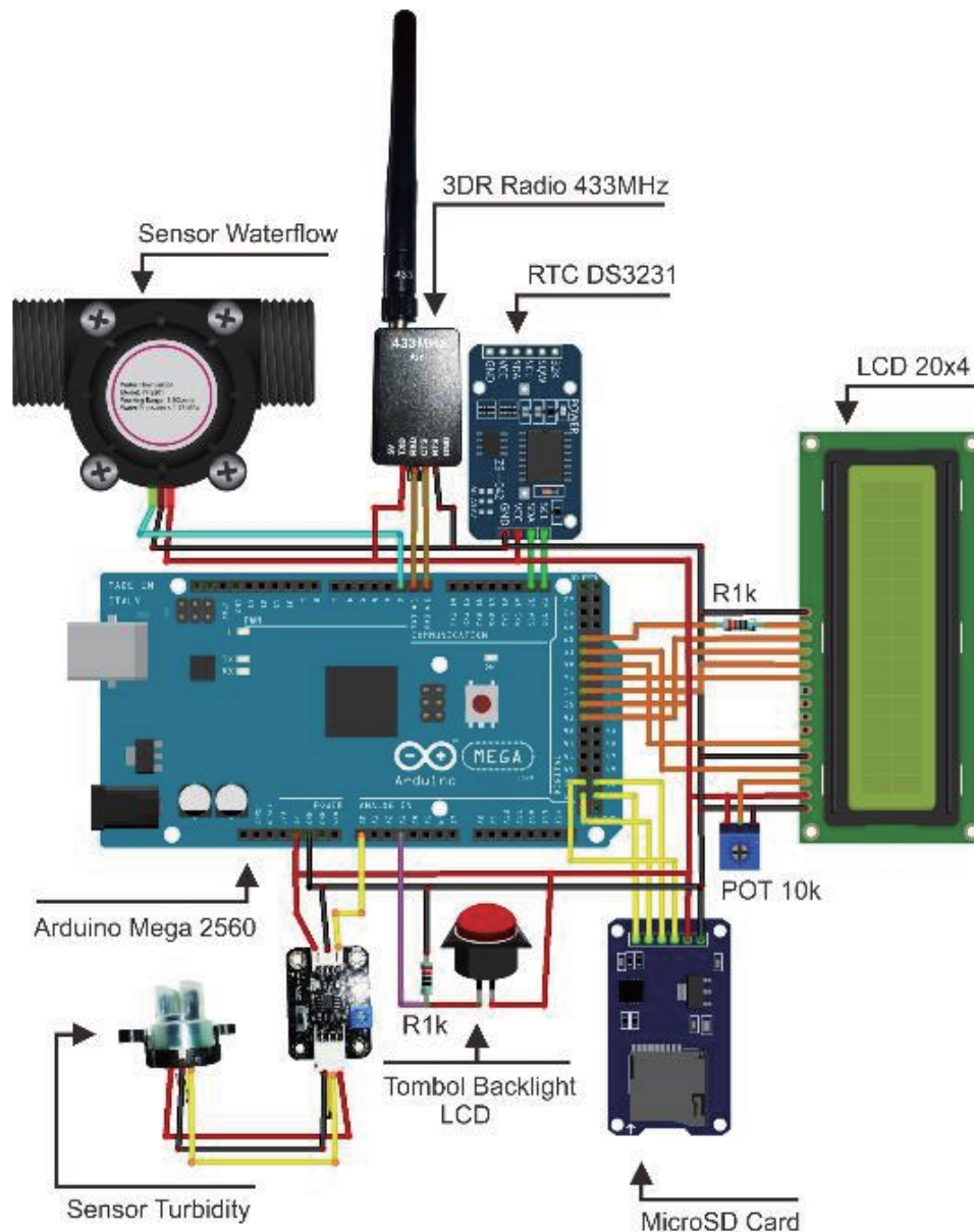
FIGURE 4. Prototype 2 design
