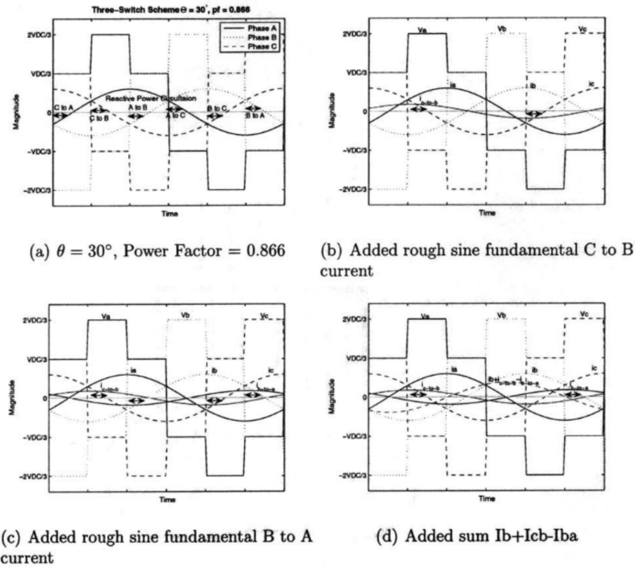
Figure 4.22: Attempt to illustrate reactive power circulation by adding the fundamental of the reactive power segments to phase B current
