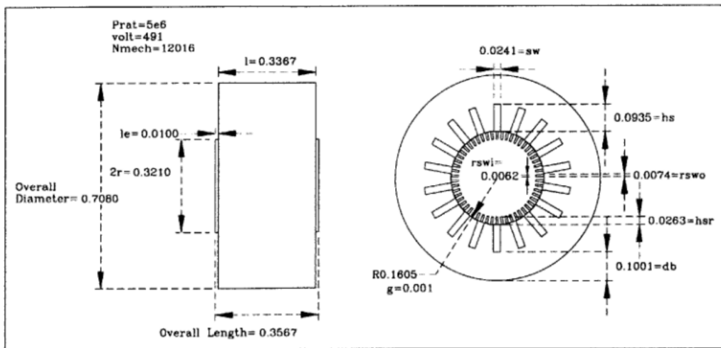
Figure 3.2: Dimensioned sketch of 5 MW generator design
