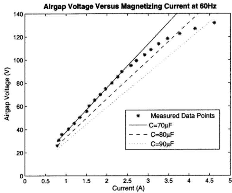
Figure 2.8: 60 Hz magnetizing current versus air gap voltage with 70, 80, and 90 \mu\text{F} capacitor slopes
