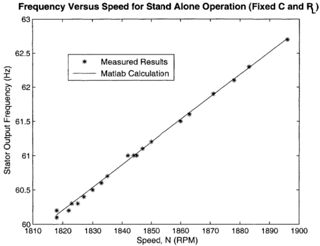
Figure 5.6: C=80\mu\text{F} , R_L = 52.5\Omega stand alone operation showing stator frequency for varied drive speed
