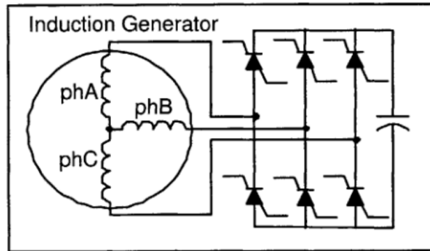
Figure 4.12: Force commutated rectifier circuit schematic
