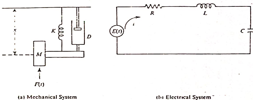
Figure 1-6. Analogy between mechanical and electrical systems.
