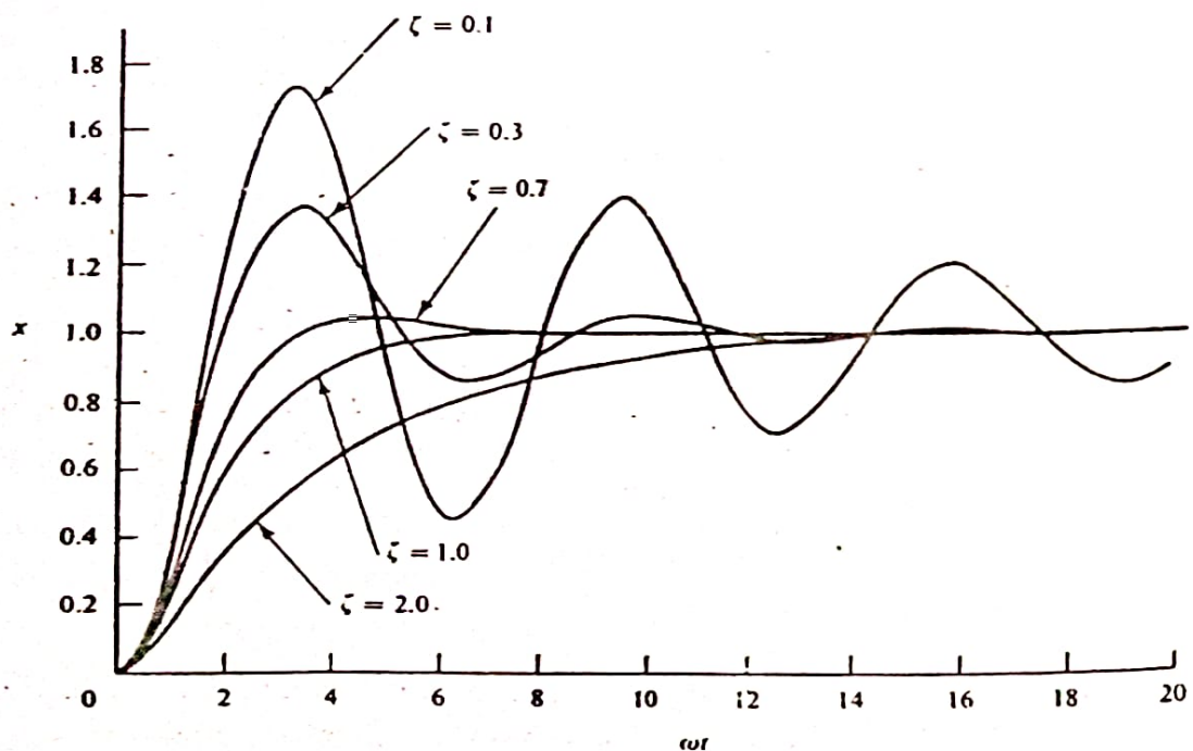
Figure 1-9. Solutions of second-order equations.
