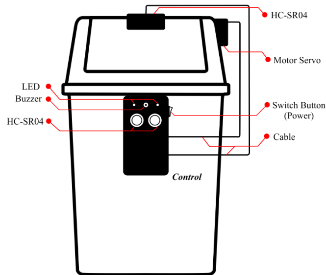
Gambar 3. 4 Modeling 2D Smart Trash
