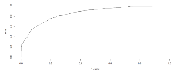
Gambar 9 Plot ROC MLP
