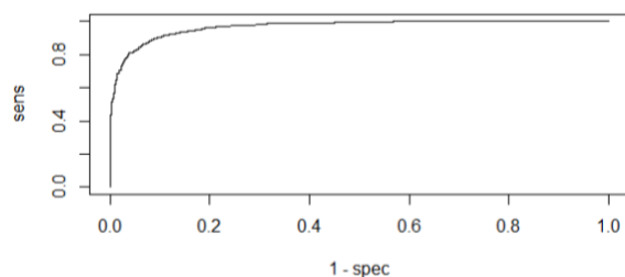
Gambar 6 plot ROC ANN
